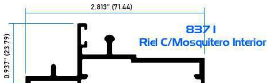
8370 Riel C/Mosquitero exterior
