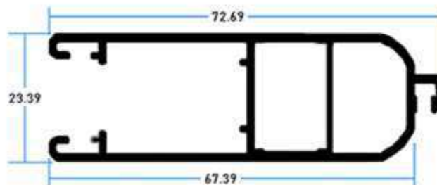
79665 Hoja Mosquitero
