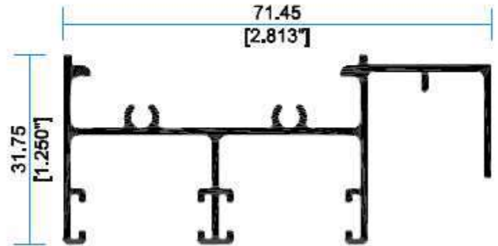
7819 Jamba C/Mosquitero
