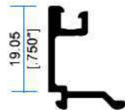
12603 Junquillo Duo
