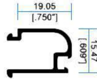
I 2576 Junquillo Colonial
