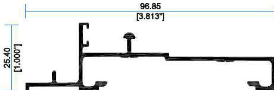
9274 Riel C/Mosquero Interior
