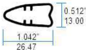
70344 Contrapeso Triangular
