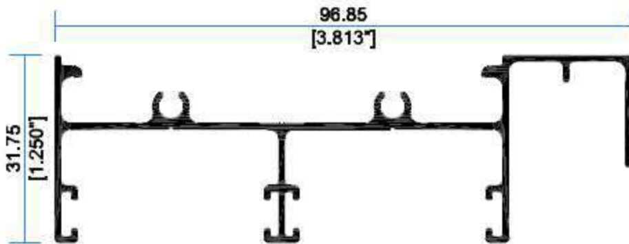
9272 Riel C/Mosquero exterior
