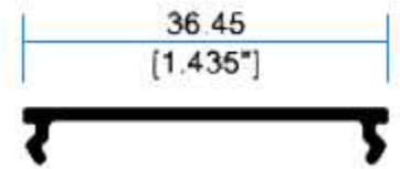
12796 Tapa Lisa
