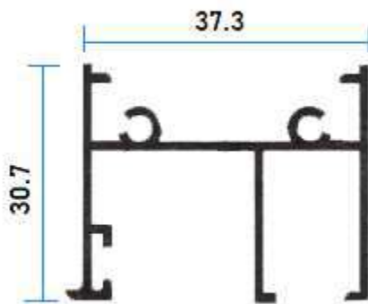
311037 Jamba
