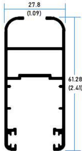
64628 Hoja Perimetral Recta
