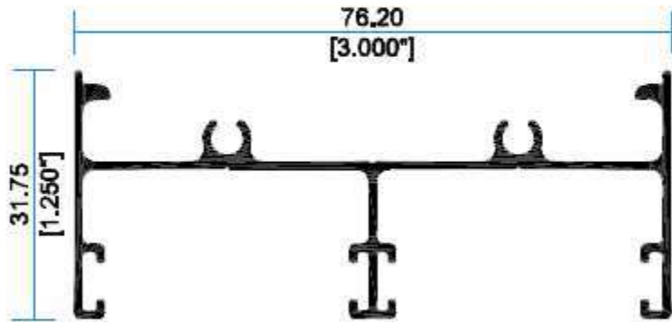
7826 Jamba
