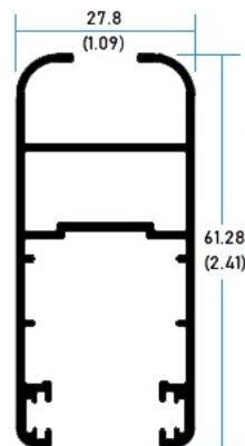
64628 Hoja Perimetral Recta
