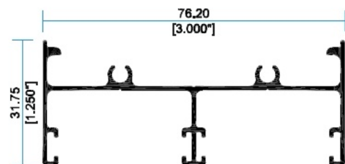
7826 Jamba
