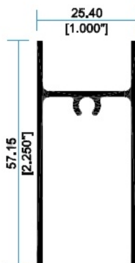
9960 Zoco Ventana Duo
