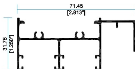
7819 Jamba C/Mosquero
