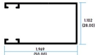
31472 Guia
