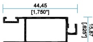
6534 Vertical
