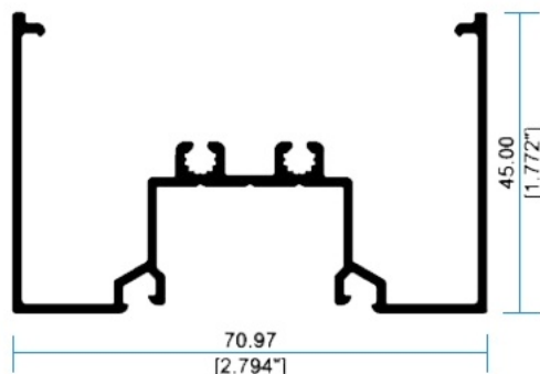
22592 Bolsa Duo
