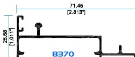
8370 Riel C/Mosquero exterior
