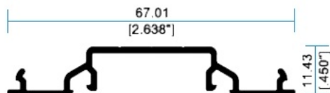
22594 Tapa Bolsa Duo
