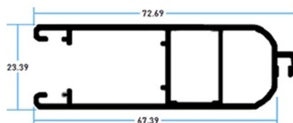
79665 Hoja Mosquitero
