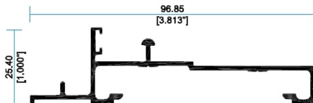
9274 Riel C/Mosquero Interior
