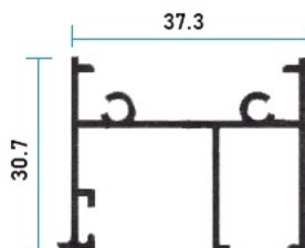
311037 Jamba
