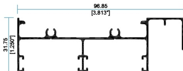
9272 Riel C/Mosquero exterior
