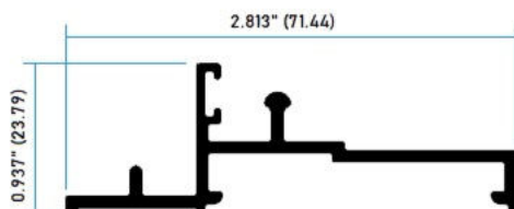
8371 Riel C/Mosquetero Interior
