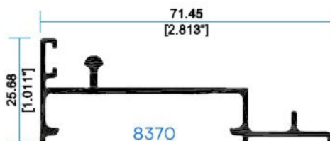
8370 Riel C/Mosquetero exterior
