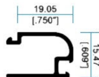
12576 Junquillo Colonial
