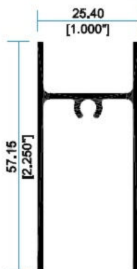
9960 Zoclo Ventana Duo
