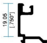
12603 Junquillo Duo
